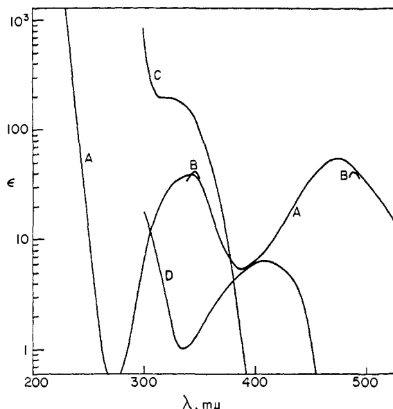
Figure 1. Absorption spectra: (A) \text{Co}(\text{NH}_3)_6\text{Cl}_3 , (B) corresponding maxima for [\text{Co}(\text{NH}_3)_5(\text{H}_2\text{O})][\text{ClO}_4]_3 , (C) benzophenone, (D) biacetyl. The latter two spectra are for 50% ethanol-water solutions.
