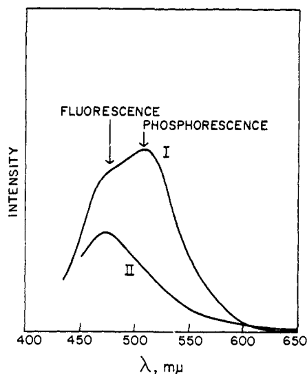
Figure 2. Emission spectra for 0.15 M biacetyl in 50% ethanol-water solution: (I) biacetyl alone; (II) with added 0.005 M \text{Co}(\text{NH}_3)_6\text{Cl}_3 .
