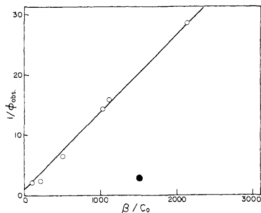
Figure 3. Data for the benzophenone-sensitized decomposition of \text{Co}(\text{NH}_3)_6^{3+} plotted according to eq 4: \circ , nondeaired solutions; \bullet , deaired solution.
